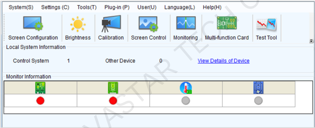
Figure 7-1 NovaLCT
