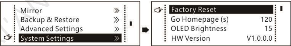
Figure 6-23 System settings
