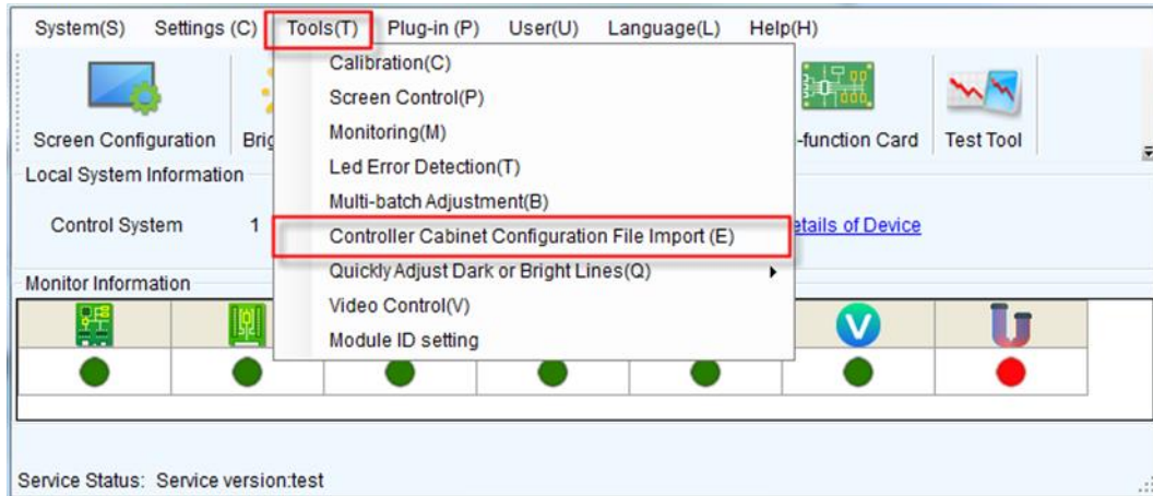
Figure 7-3 Home page
