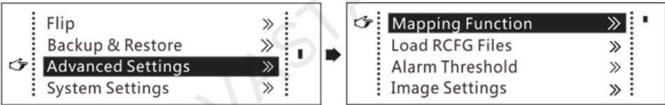
Figure 6-20 Mapping function
