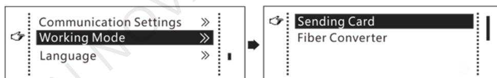
Figure 6-25 Working mode
