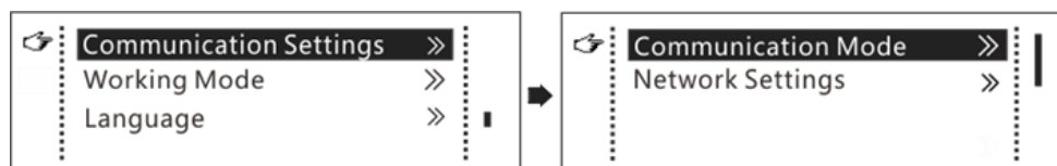
Figure 6-24 Communication mode
