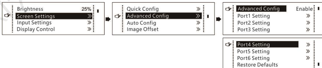
Figure 6-7 Advanced configuration
