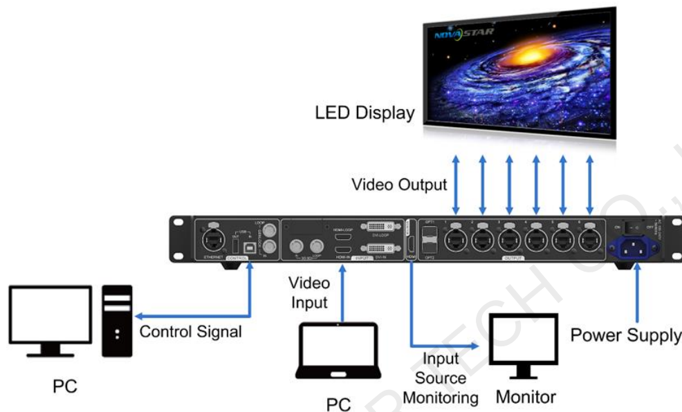
Figure 3-1 Application of sending card mode
