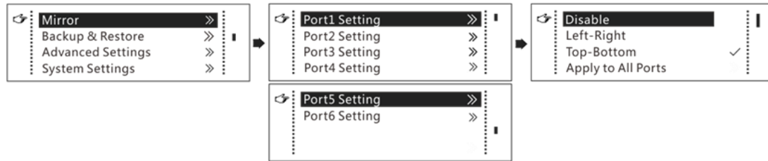
Figure 6-13 Image mirroring
